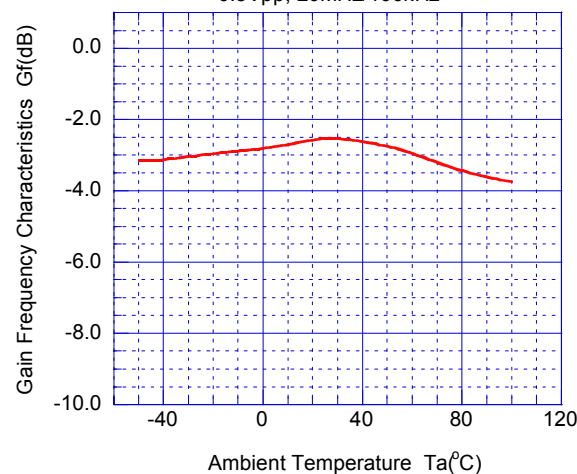
Gain Frequency Characteristics vs. Temperature (Bias+Through Type Input) 0.5Vpp, 20MHz/100kHz
